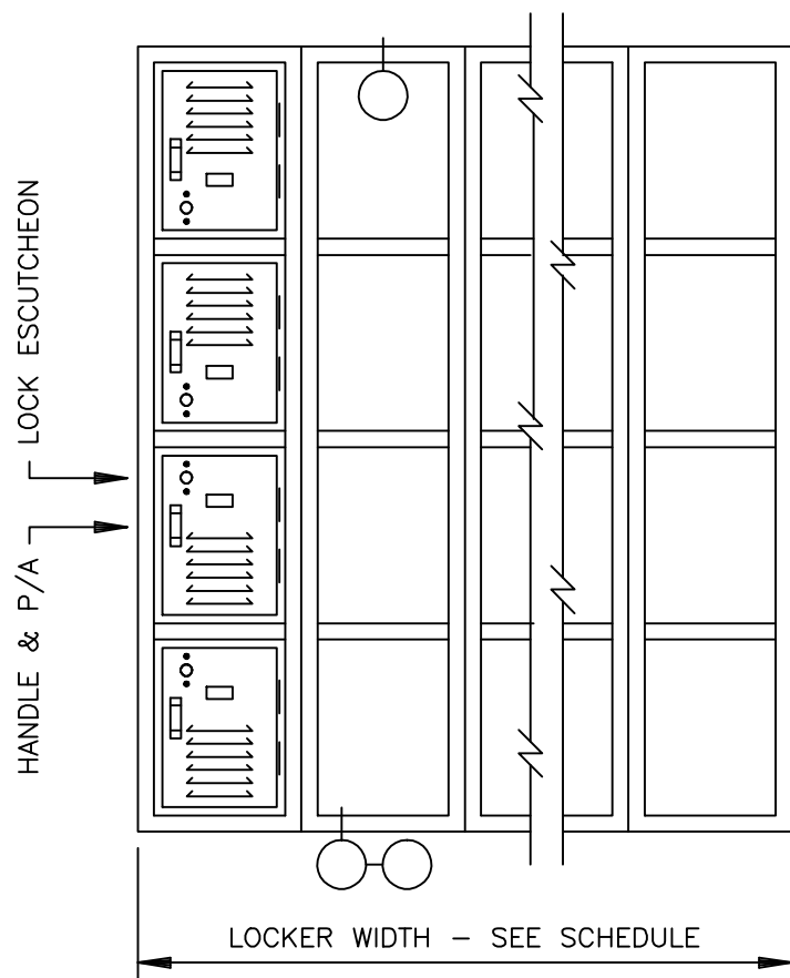
FRONT ELEVATION
