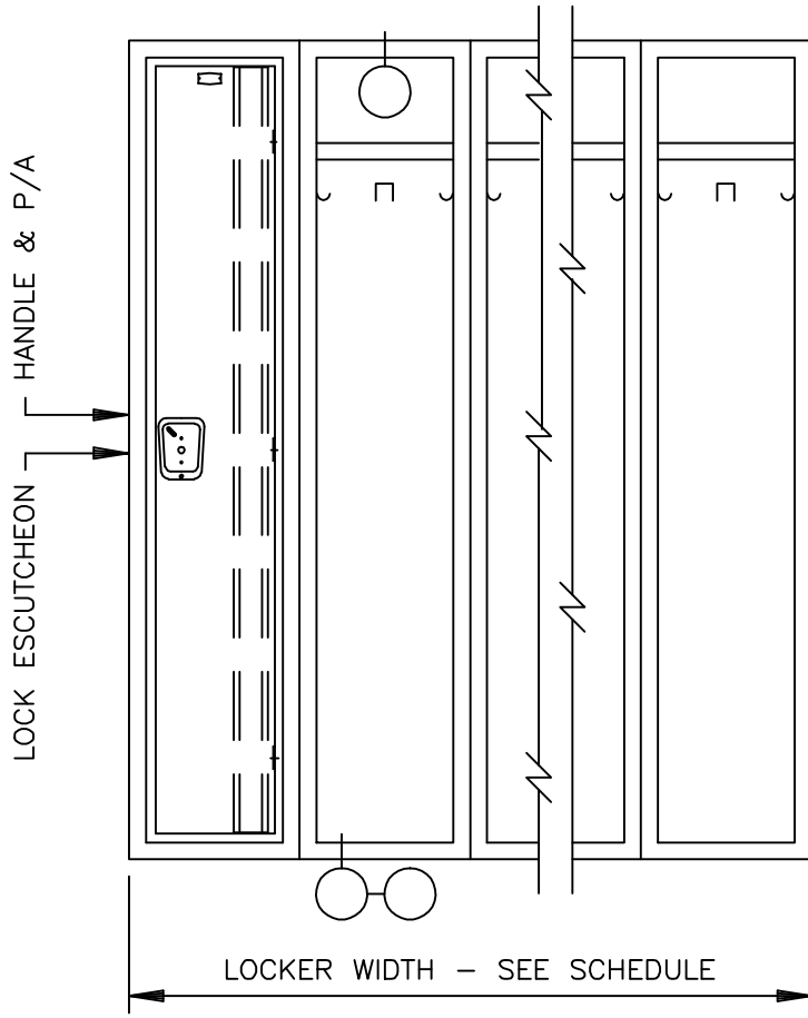
FRONT ELEVATION
