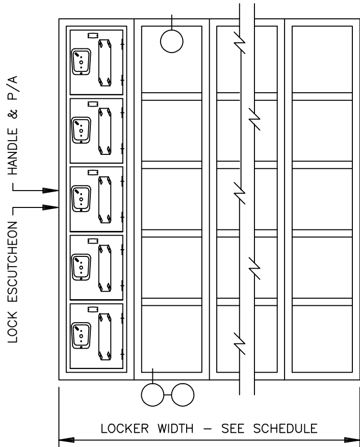
FRONT ELEVATION
