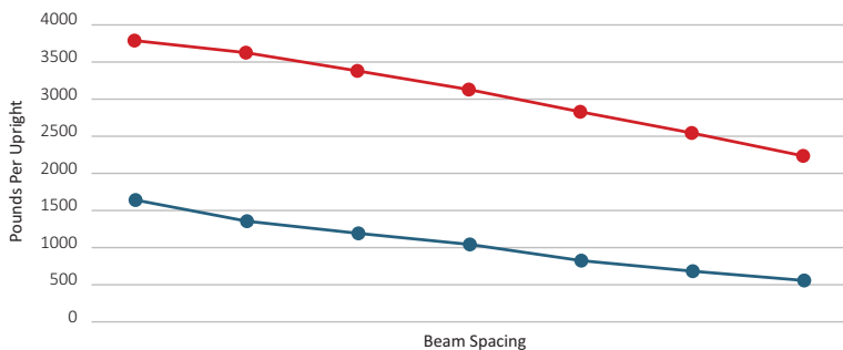
Rivet Rack Static Post Capacity
