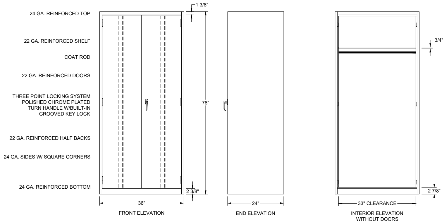
1200 SERIES WARDROBE CABINET KNOCK DOWN CAT# RS1296 36"W x 24"D x 78"H W/ 1 SHELF & COAT ROD COLOR: 20-DOVE GRAY
