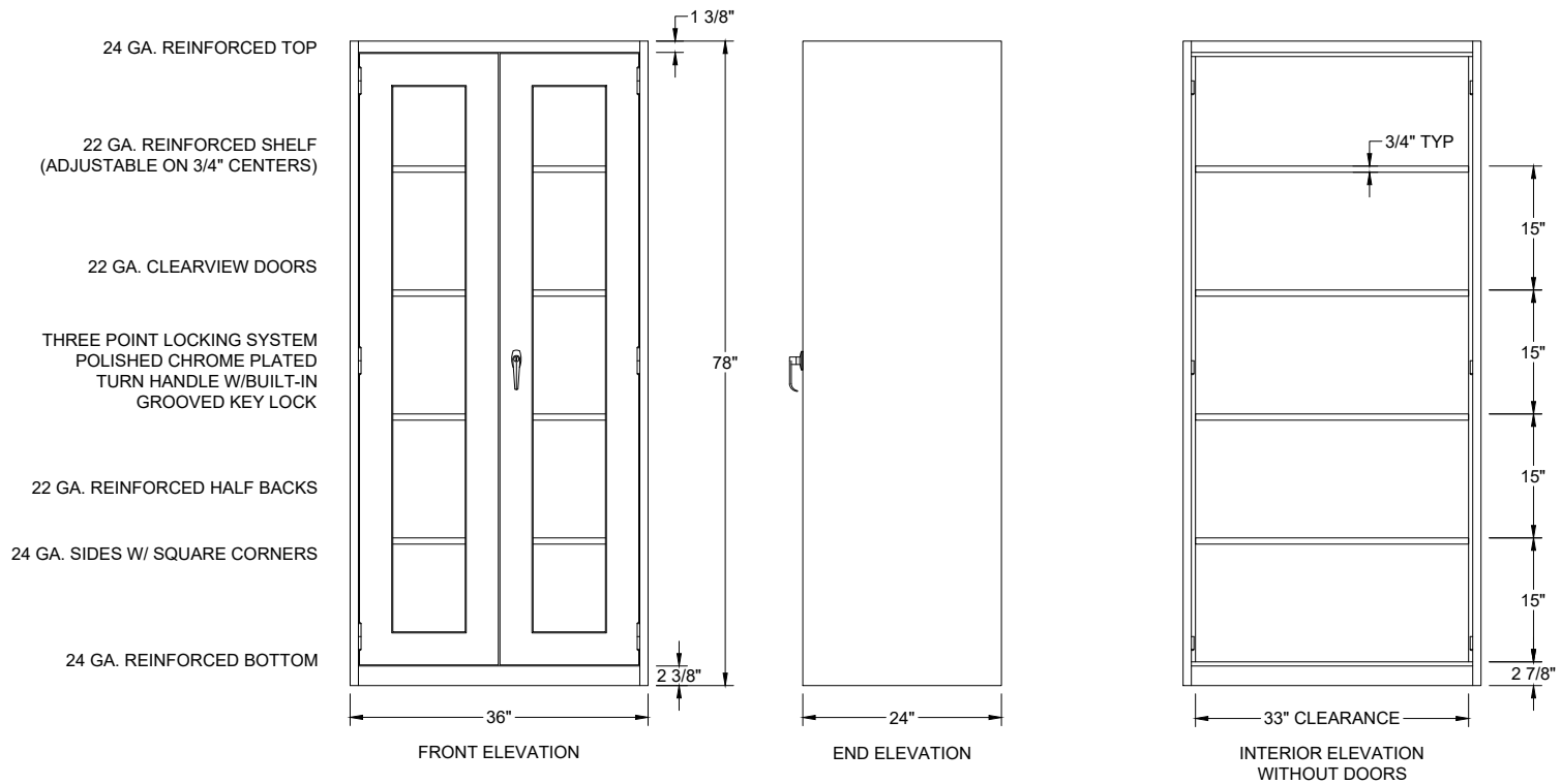
1200 SERIES VISIBLE STORAGE CABINET KNOCK DOWN CAT# RS1291V 36"W x 24"D x 78"H W/ 4 SHELVES & VISIBLE DOORS COLOR: 20-DOVE GRAY
