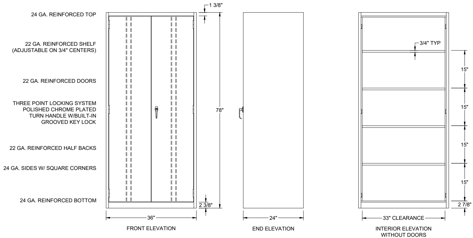
1200 SERIES OFFICE CABINET KNOCK DOWN CAT# RS1291 36"W x 24"D x 78"H W/ 4 SHELVES COLOR: 20-DOVE GRAY
