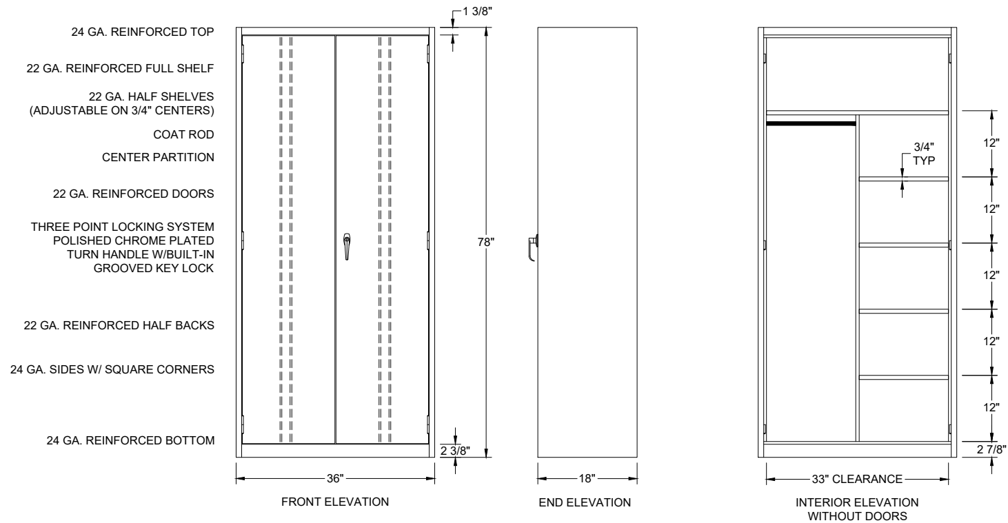
1200 SERIES COMBINATION WARDROBE CABINET ASSEMBLED CAT# RS1288 36"W x 18"D x 78"H W/ 1 FULL SHELF, 4 HALF SHELVES & COAT ROD COLOR: 20-DOVE GRAY
