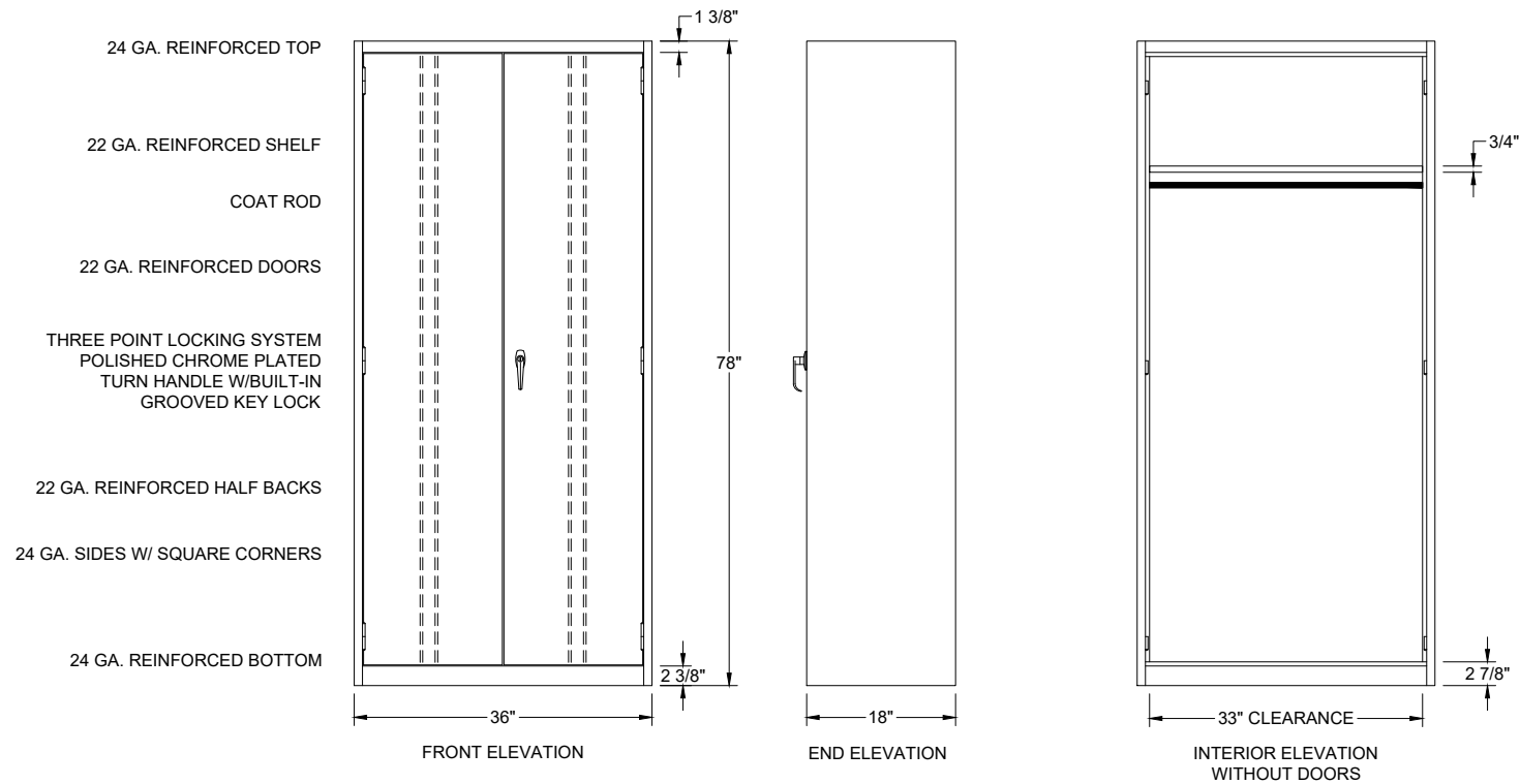
1200 SERIES WARDROBE CABINET KNOCK DOWN CAT# RS1286 36"W x 18"D x 78"H W/ 1 SHELF & COAT ROD COLOR: 20-DOVE GRAY
