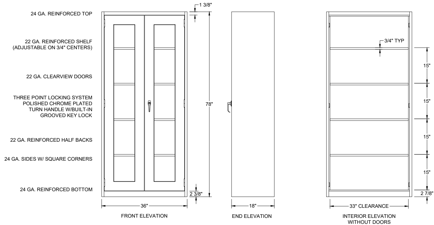
1200 SERIES VISIBLE STORAGE CABINET ASSEMBLED CAT# RS1280V 36"W x 18"D x 78"H W/ 4 SHELVES & VISIBLE DOORS COLOR: 20-DOVE GRAY
