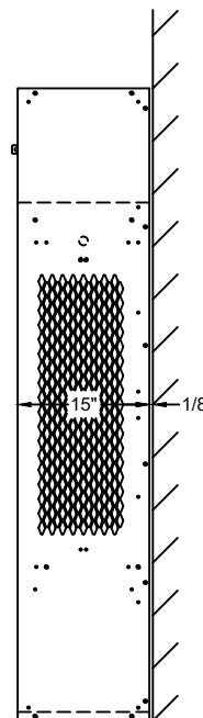
SINGLE ROW END ELEVATION
