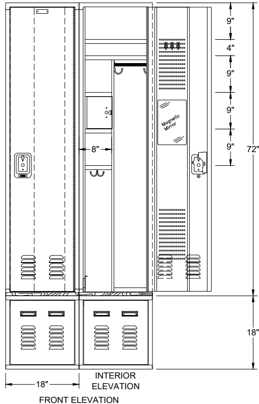
WELDED LAW ENFORCEMENT LOCKER FRAMES 18" X 24" X 72" S.R.S.T. W/ WELDED LOWER COMPARTMENT 18" X 36" X 18"
