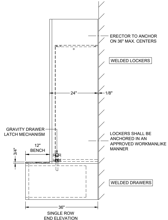
WELDED LAW ENFORCEMENT LOCKER FRAMES 18" X 24" X 72" S.R.S.T. W/ WELDED LOWER COMPARTMENT 18" X 36" X 18"
