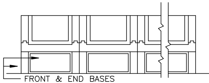
PARTIAL FRONT ELEVATION
