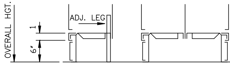
SR SECTION
