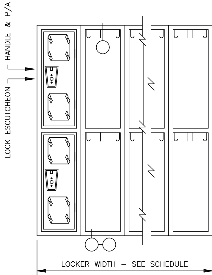
FRONT ELEVATION
