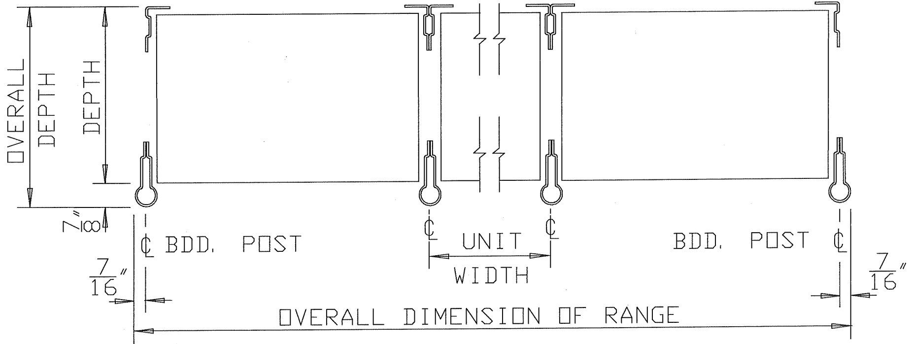
TYPICAL LAYOUT OF BEADED POST RANGE (S. F. RANGE SHOWN)
