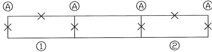
STANDARD SINGLE ROW BRACING PATTERN REFERENCE 'TYPICAL BACK BRACE' FOR '1' & '2' BRACING LOCATIONS REFERENCE 'TYPICAL SIDE BRACE' FOR 'A' & 'B' BRACING LOCATIONS
