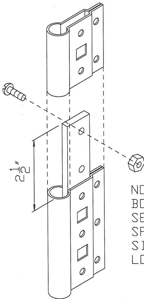
ISOMETRIC VIEW SHOWING BEADED POST SPLICE
