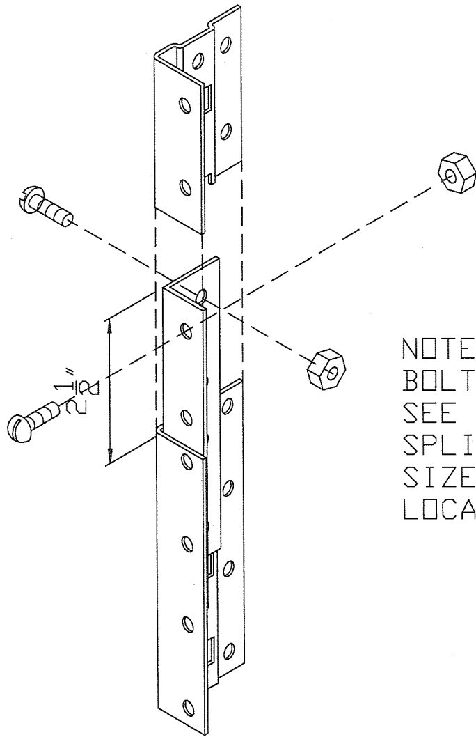
ISOMETRIC VIEW SHOWING ANGLE POST SPLICE
