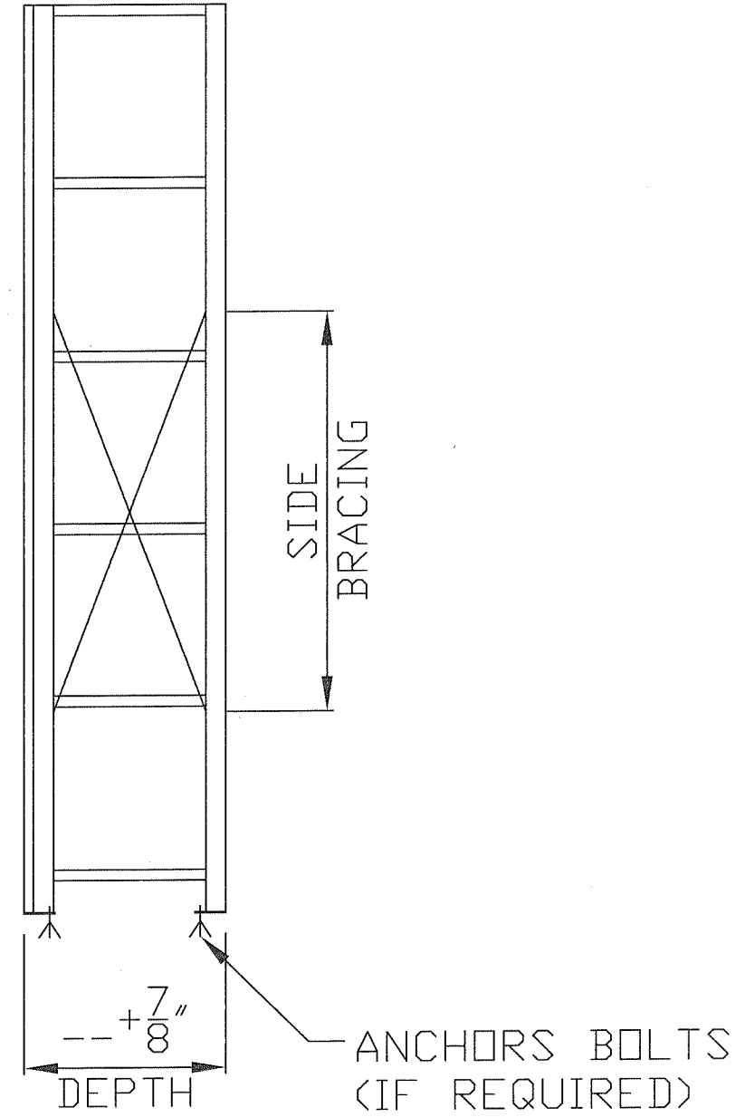
SIDE VIEW ELEVATION
