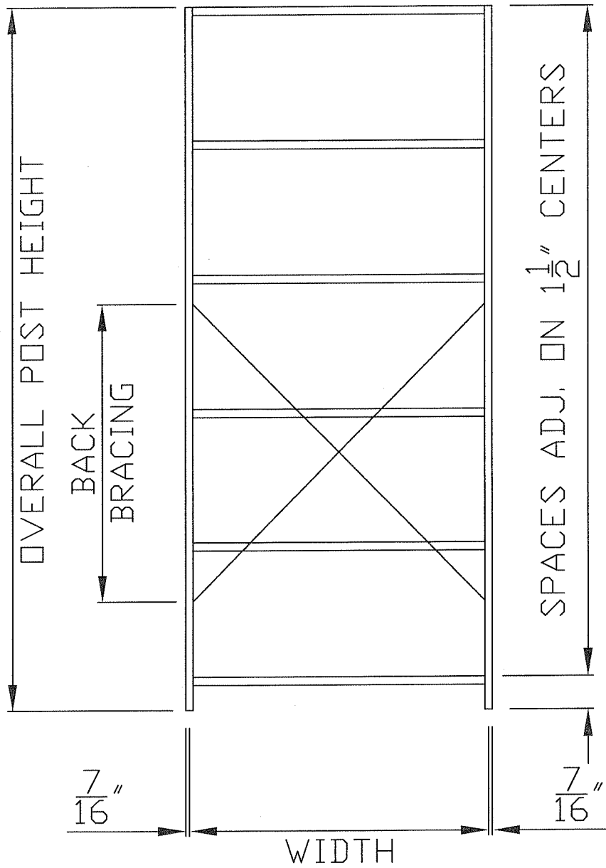
FRONT VIEW ELEVATION
