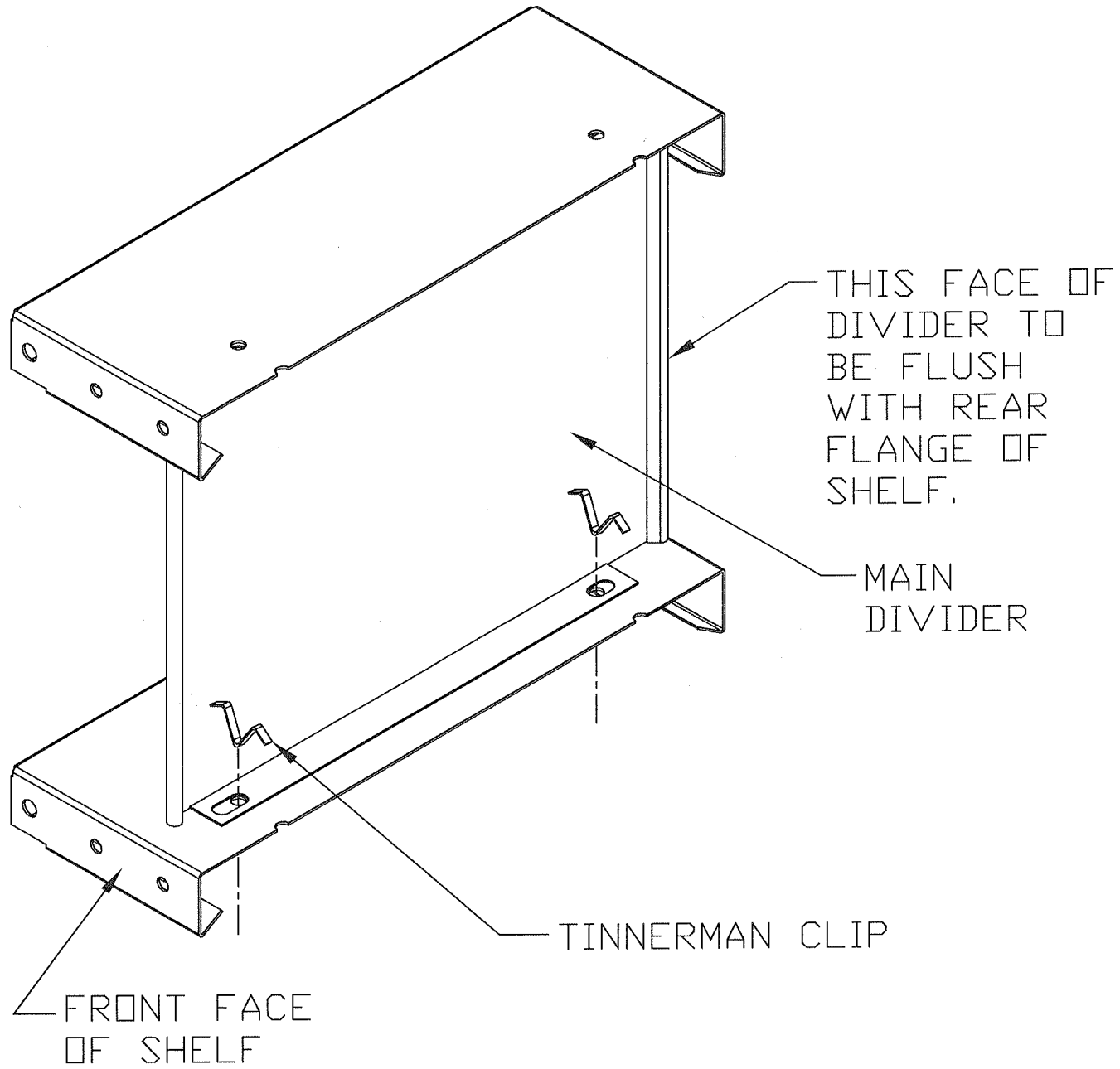
ATTACHMENT OF FULL HEIGHT SHELF DIVIDER TO OPEN FLANGE SHELF
