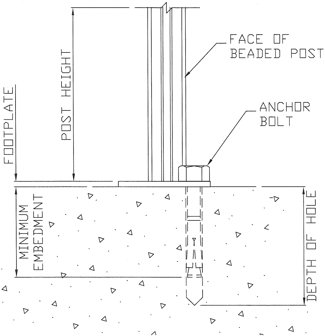
TYPICAL BEADED POST FOOTPLATE ANCHORAGE
