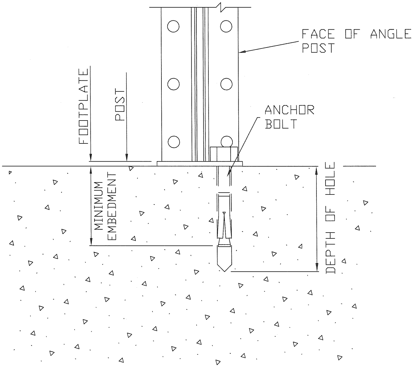
TYPICAL ANGLE POST FOOTPLATE ANCHORAGE
