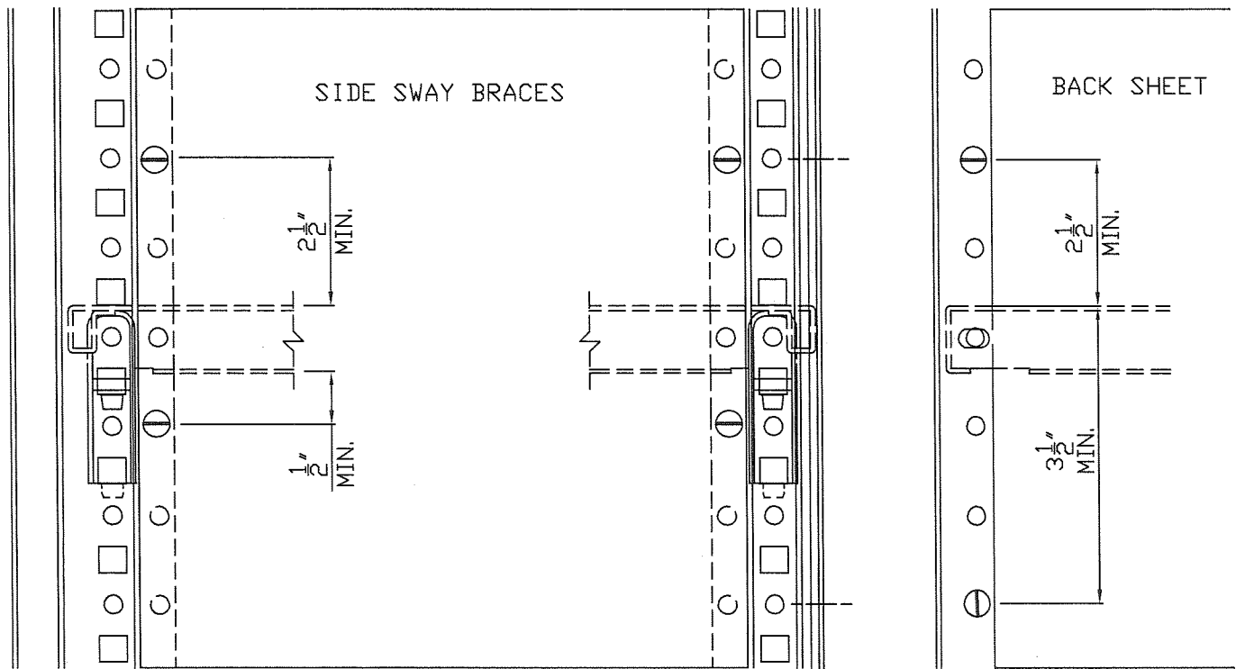
CONNECTION DETAIL: BEADED POST UPRIGHT SHEET CONNECTION (W/BOX SHELF)
