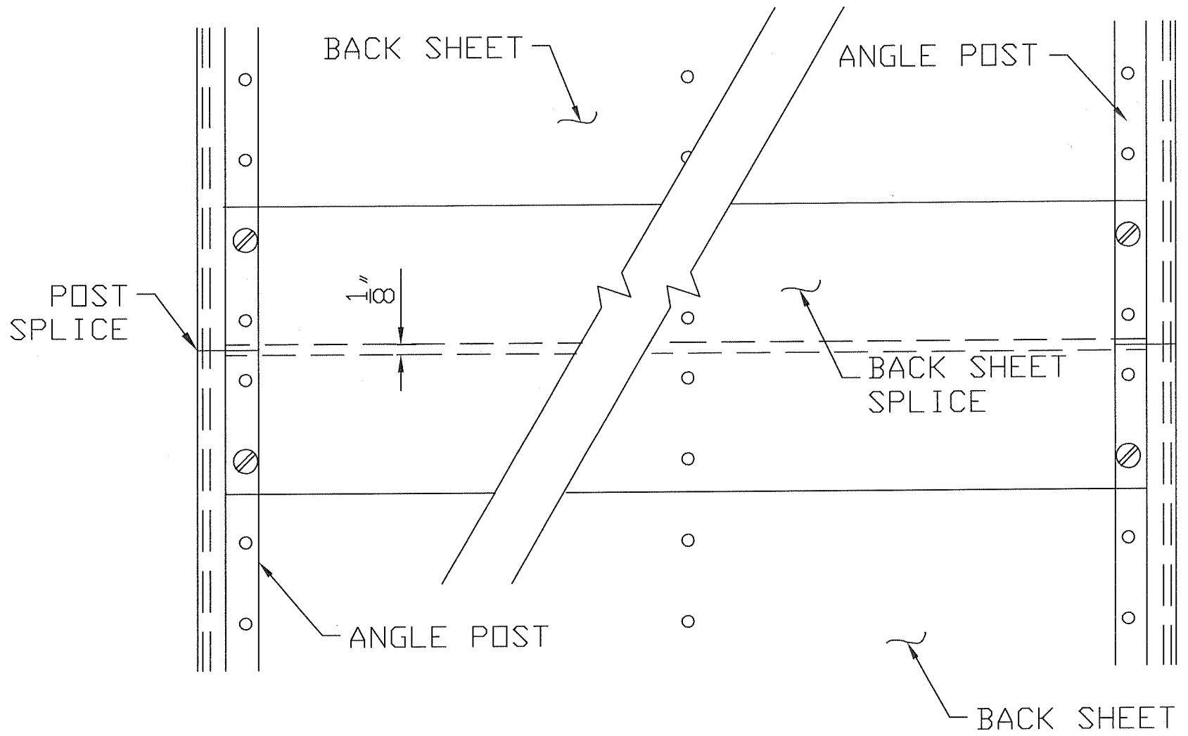
CONNECTION DETAIL ANGLE POST BACK SPLICE
