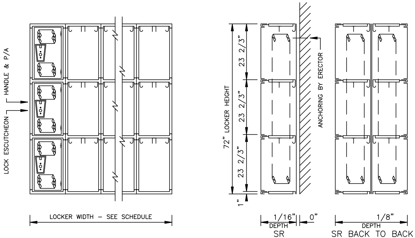
ALL WELDED VENTILATED TRIPLE TIER LOCKER (72" FRAME)
