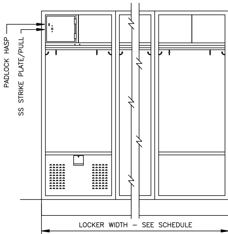
FRONT ELEVATION
