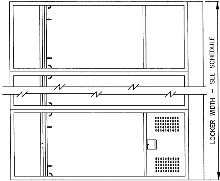
SECTION SR. FRONT ELEVATION HEAVY DUTY VENTILATED MVP (OPEN FRONT LOCKER) WITH FOOTLOCKER
